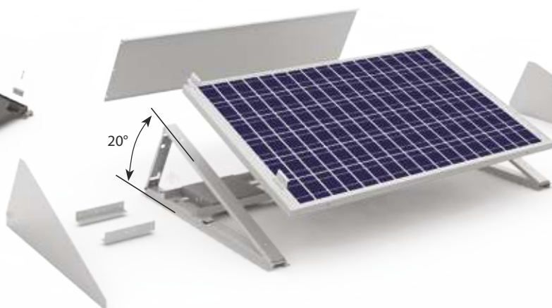
Solarstell ballast in bodem
